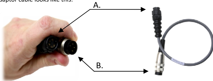
A. 5-pin Female Switchcraft Connector B. 4-pin Male Lumberg Circular Din Connector
