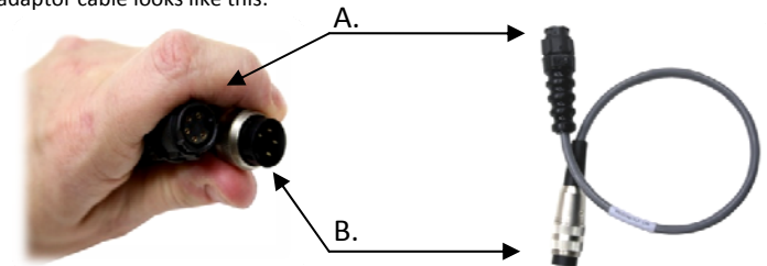
A. 5-pin Female Switchcraft Connector B. 4-pin Male Lumberg Circular Din Connector
